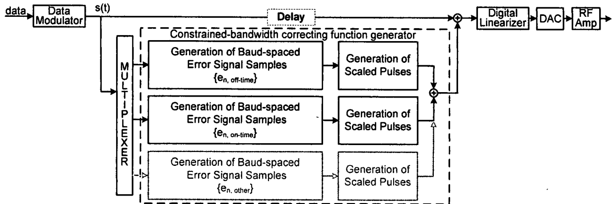
Figure 2. Functional Architecture of the Peak-Reduction Approach of U.S. App. Ser. No. 10/718,507
